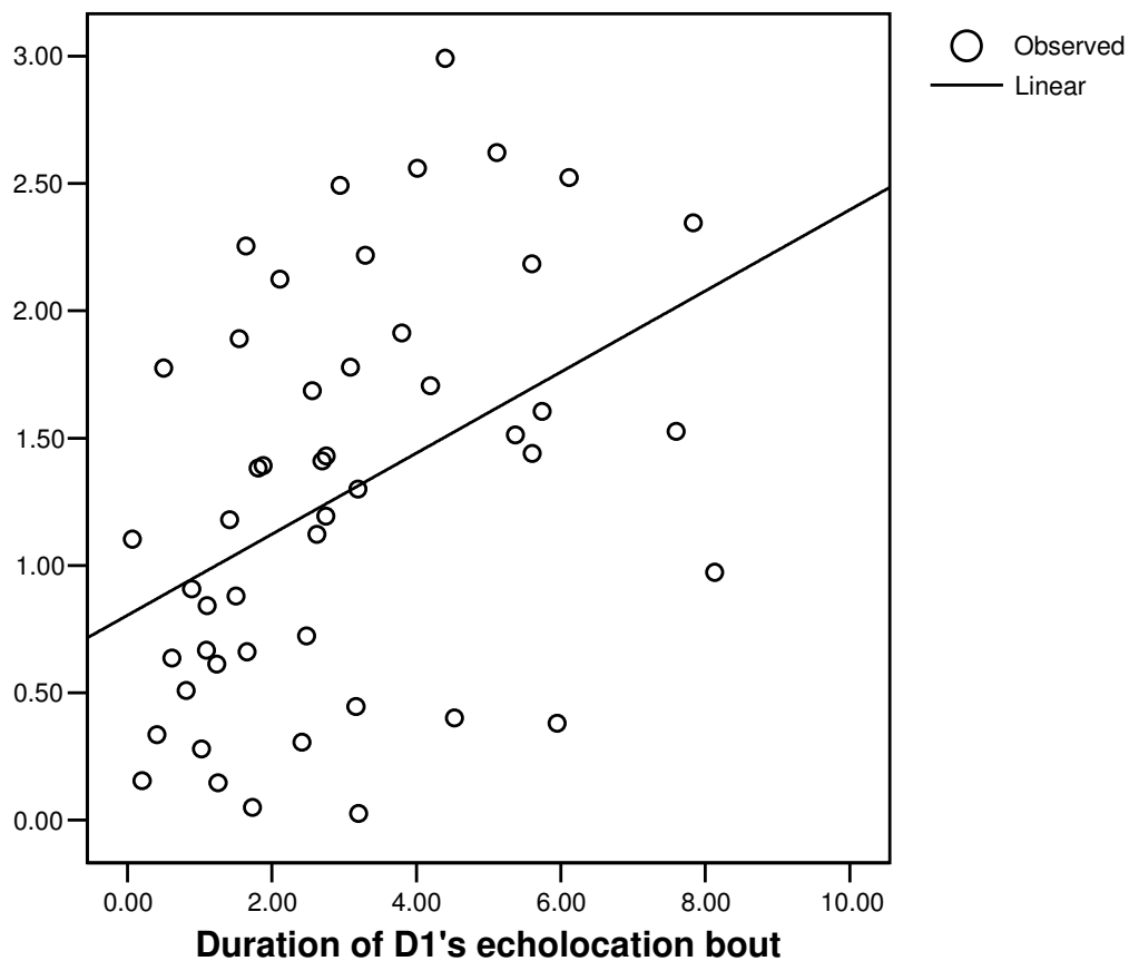
Figure 4.3.3 Regression of duration D1's echolocation bout vs. delay between D1 and D2's echolocation
