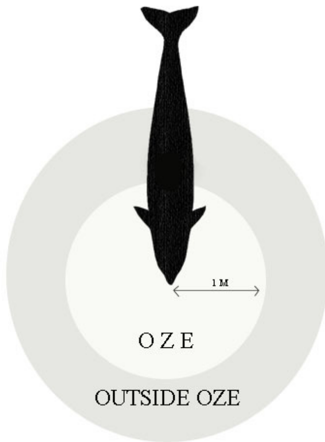
Figure 5.1.2 OZE relative to dolphin length
