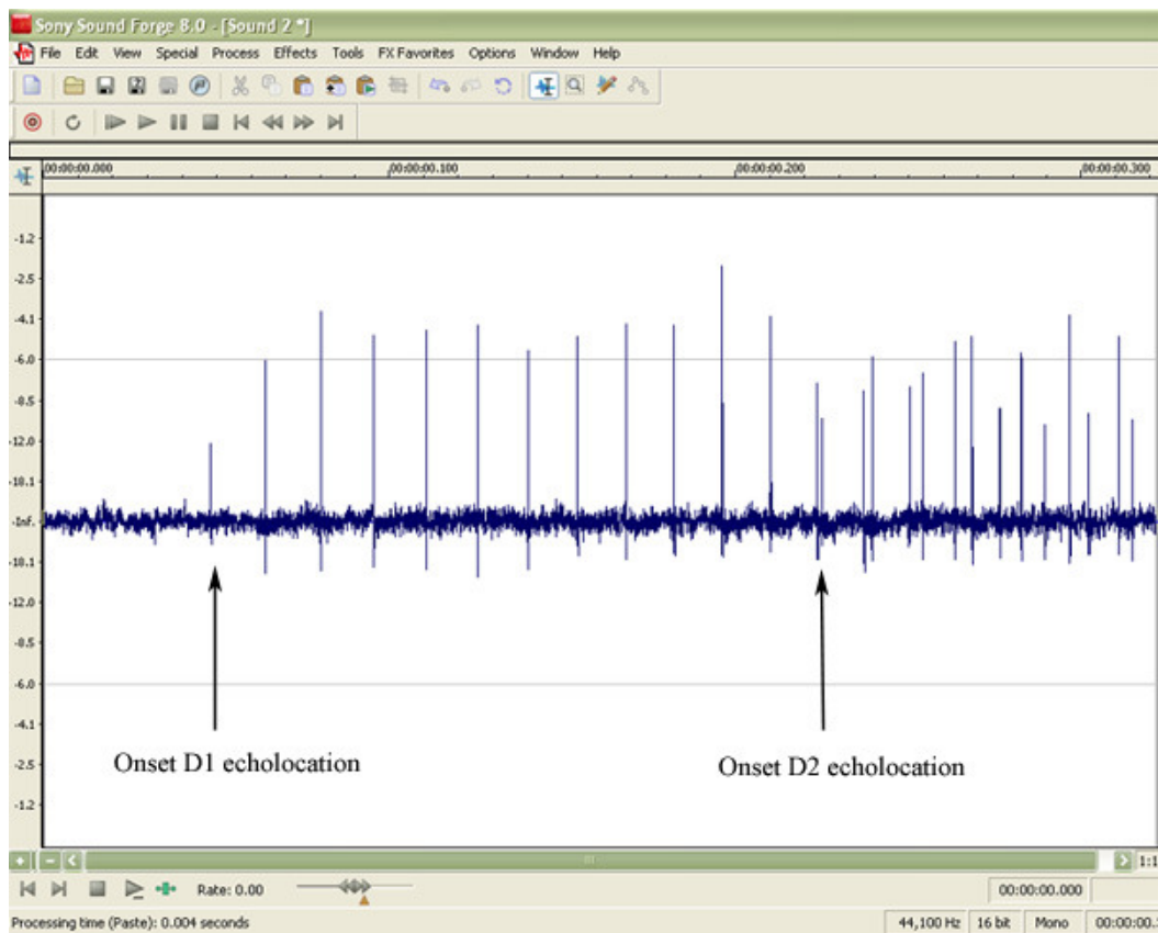
Figure 3.3.2 Waveform showing onset of D1 and D2 echolocation clicktrains
