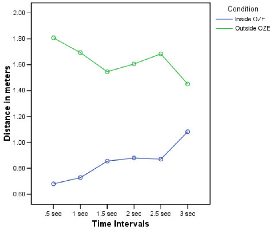
Figure 5.2.2 Plot showing changes in distance for each conditions (inside vs. outside OZE) across time
