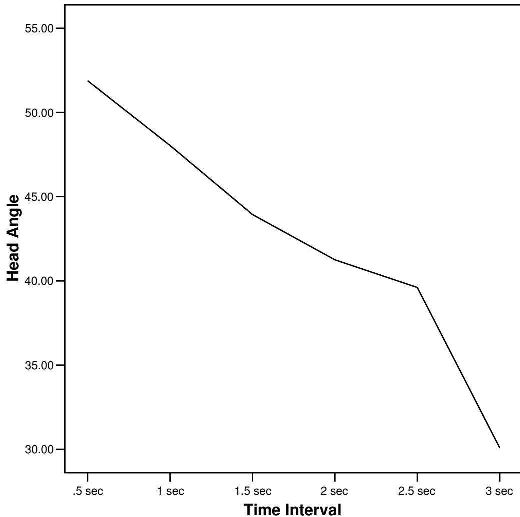
Figure 5.3.3 Plot of changes in mean head angle across time for all dolphins– starting at ‘.5 sec’ instead of ‘start of event’
